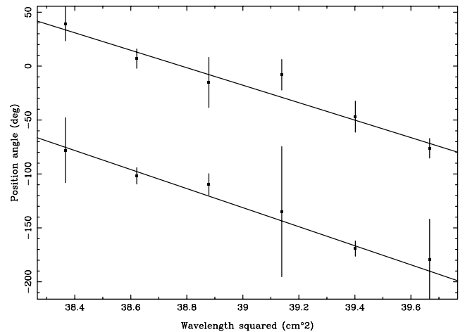
Figure 4. Position angle versus \lambda^2 across the 4.8-GHz band on September 1 for the first (top) and second (bottom) components. The position angle separation between the components is near 110^\circ , as expected. The straight lines show the fit to the data from which the RM can be derived.
