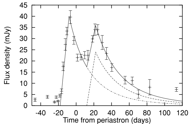
Figure 6. Flux density of the unpulsed emission at 1.4 GHz. Superposed is the solution to the model described in the text. The model includes a rise time of 10 d and adiabatic expansion for each of the synchrotron bubbles created in the disc crossings. The dashed lines indicate the light curve for each bubble individually. The solid line is the sum of both light curves.
