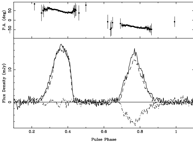
Figure 1. Mean pulse profile at 1.4 GHz. Position angle is shown on top, and the total intensity (solid line), linear (dashed line) and circular (dash-dot line) polarizations are shown in the bottom panel.
